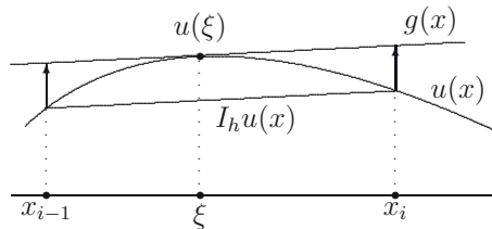
Abbildung 11.2: Lineare Approximation
